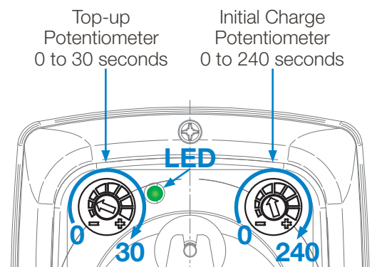
Model D1TT: Top-up and Initial Charge
