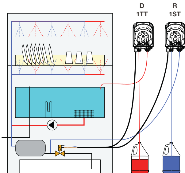
Wiring Example - Single-Valve Dish Machine
