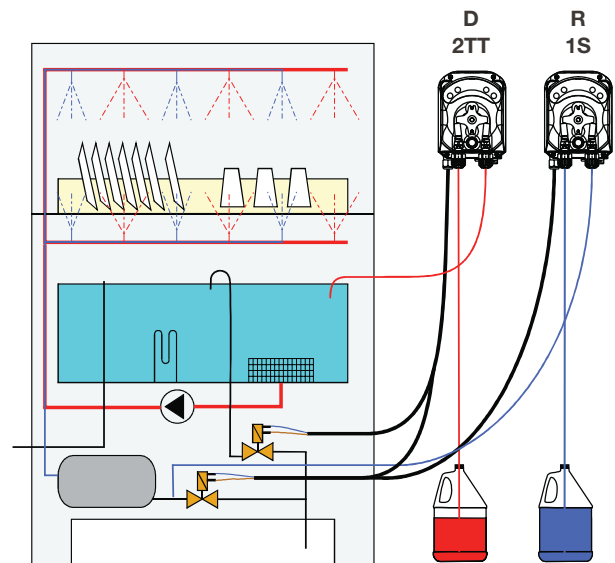
Wiring Example - Two-Valve Dish Machine
