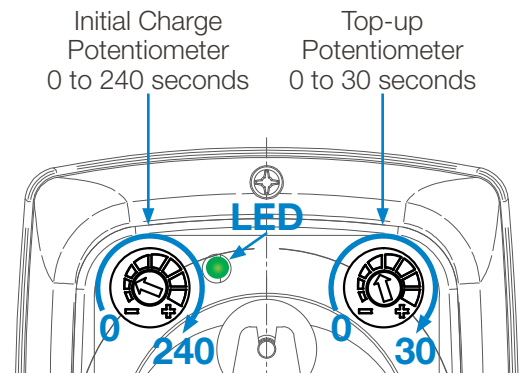
Model D2TT: Initial Charge and Top-up
